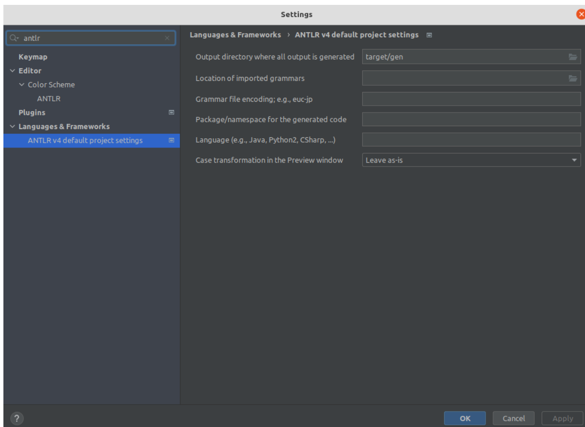
图 29: Configure ANTLR plugin
