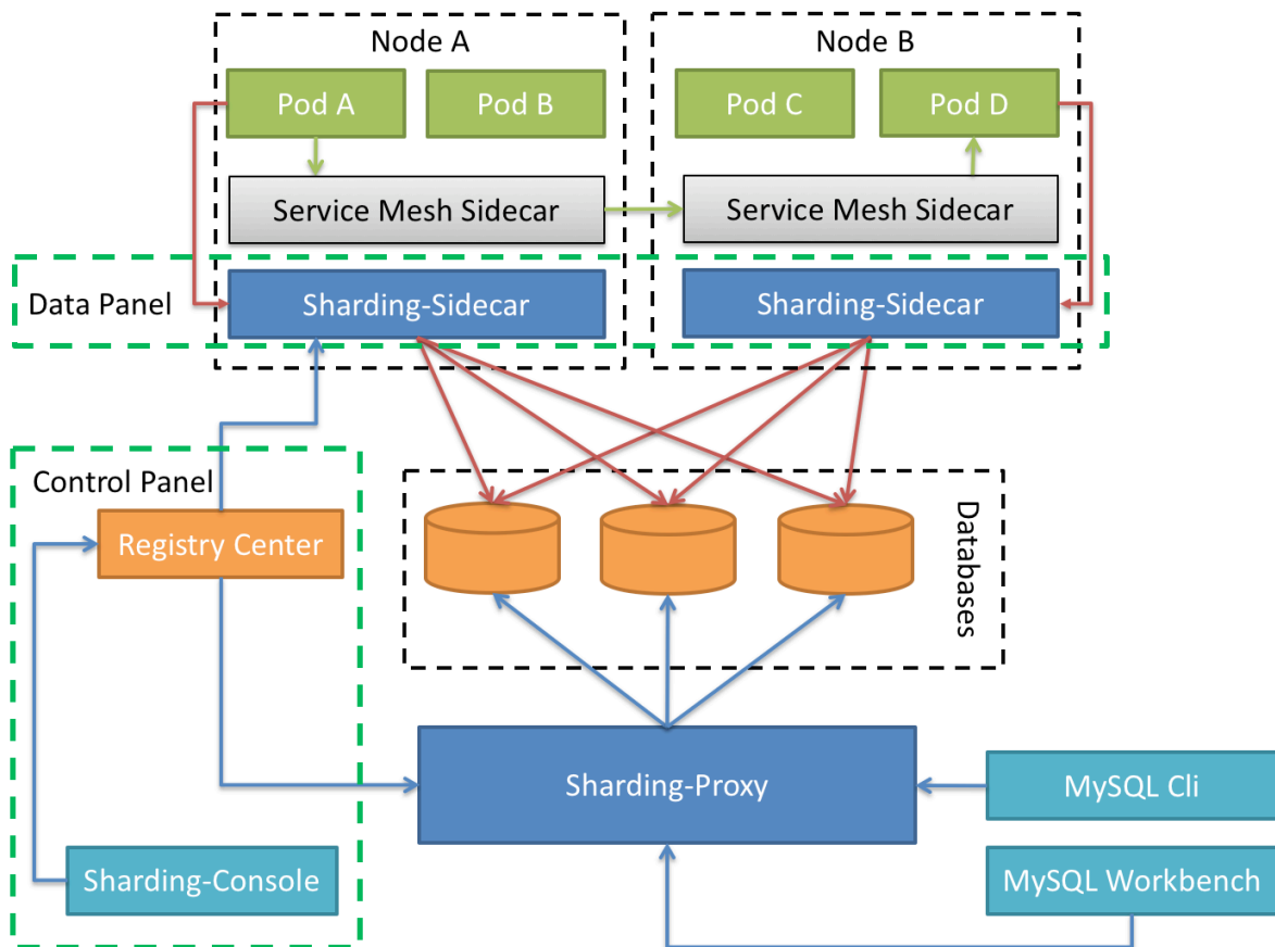
图 3: ShardingSphere-Sidecar Architecture
