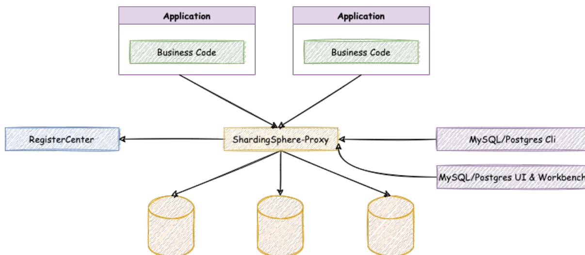
图 2: ShardingSphere-Proxy Architecture
