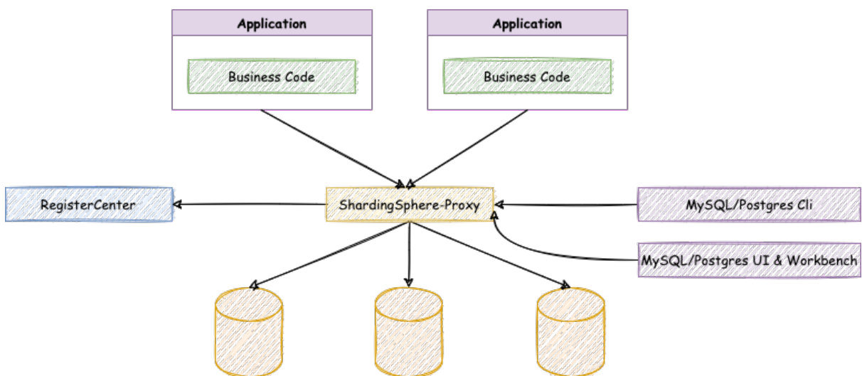
图 2: ShardingSphere-Proxy Architecture
